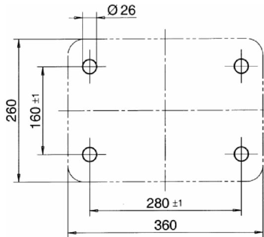
Fig. A1 Buffer supporting plate
