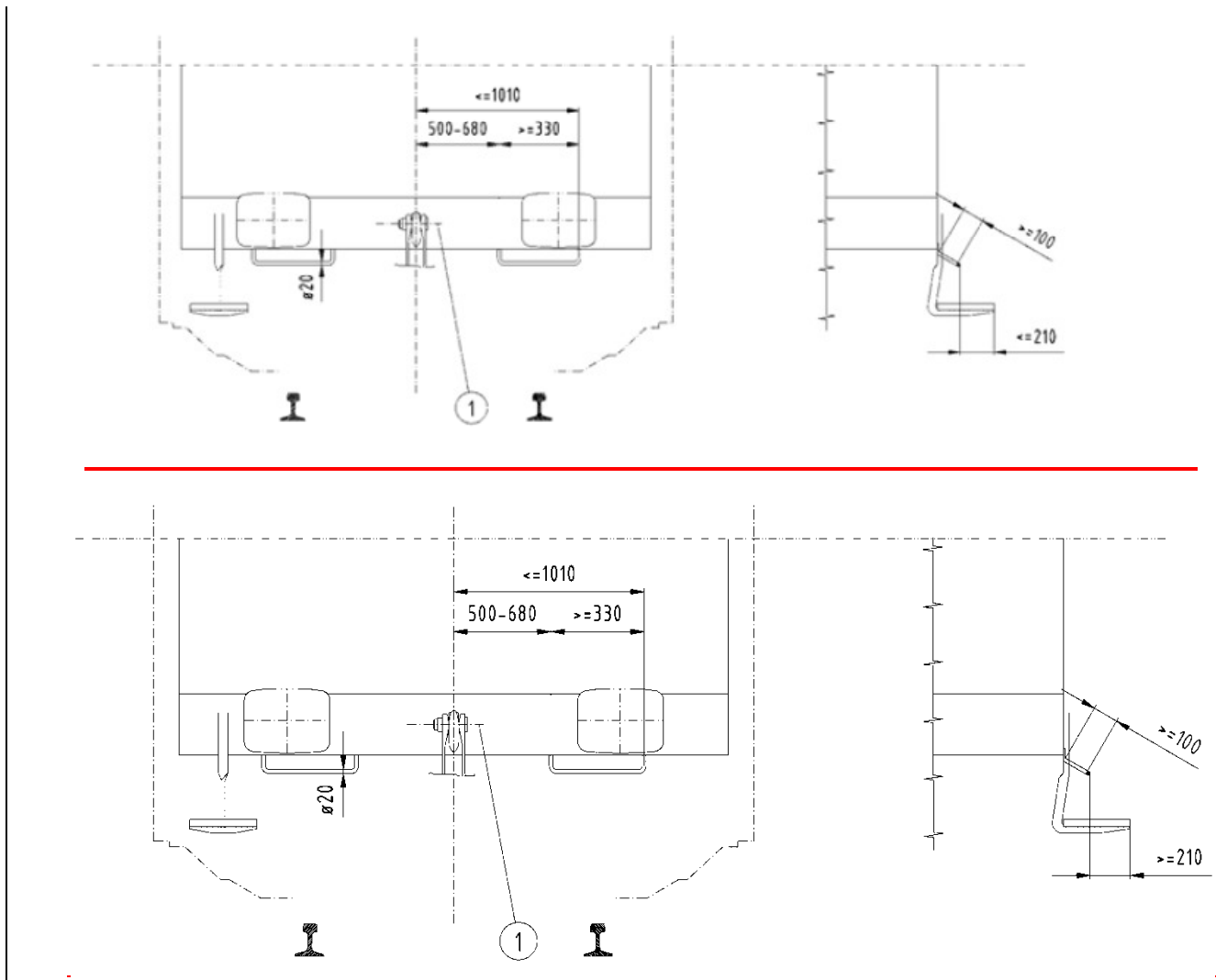
Figure 7: Positions of shunter handrails [d17]
