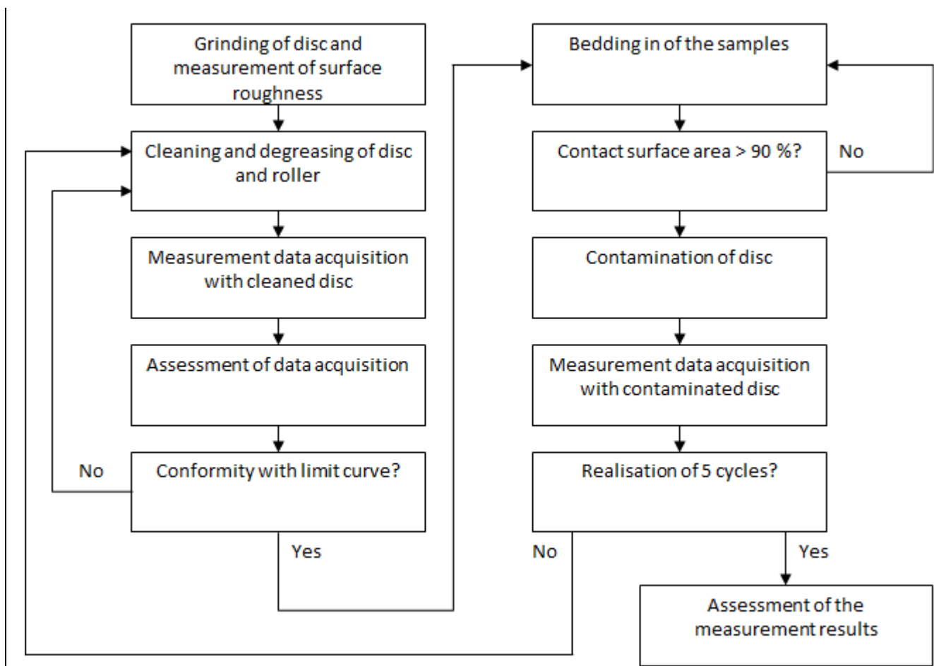
Figure 4: Flow chart of the test program
