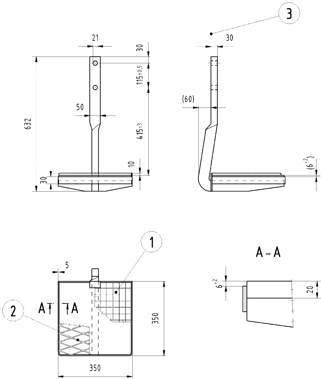
Figure 4: Shunter's step
